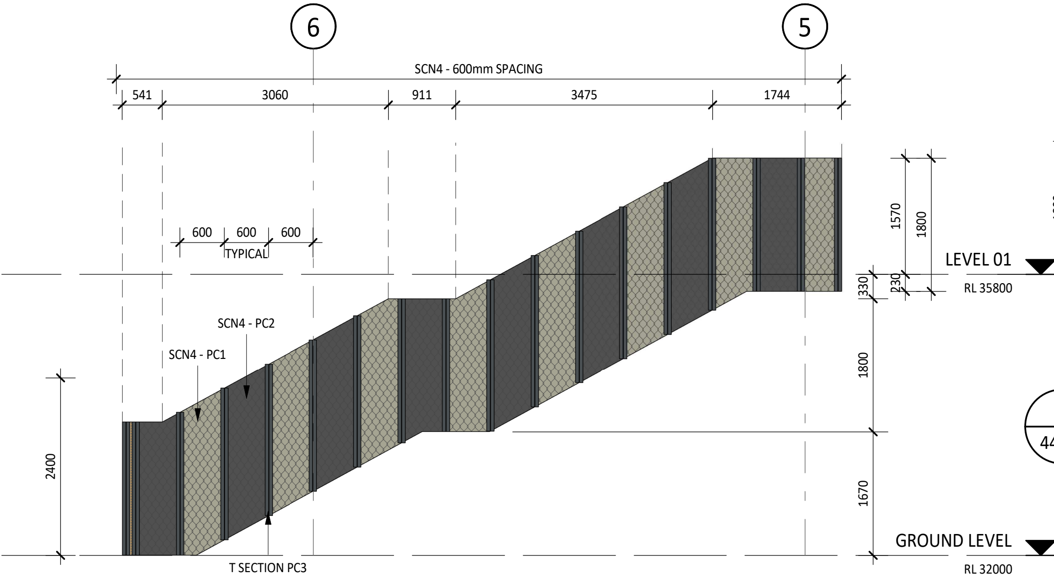
2 EXTERNAL STAIR SCREEN ELEVATION 44-02 1 : 50
