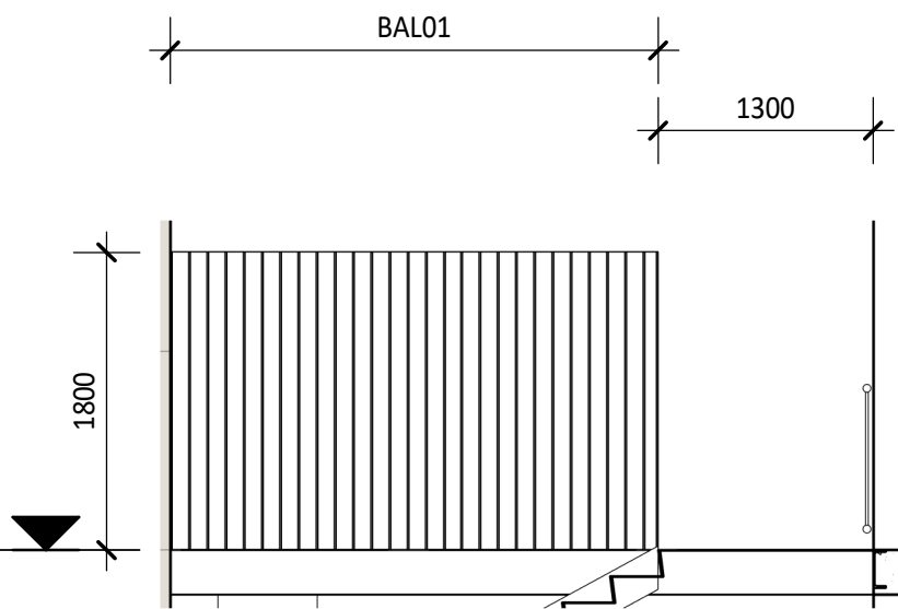
3 EXTERNAL STAIR SCREEN ELEVATION 44-03 1 : 50
