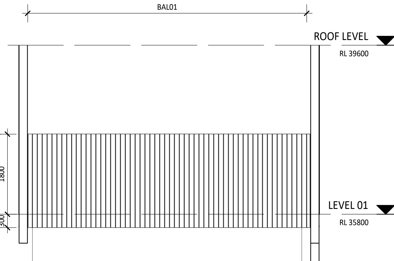
5 EXTERNAL STAIR SCREEN ELEVATION 44-03 1 : 50
