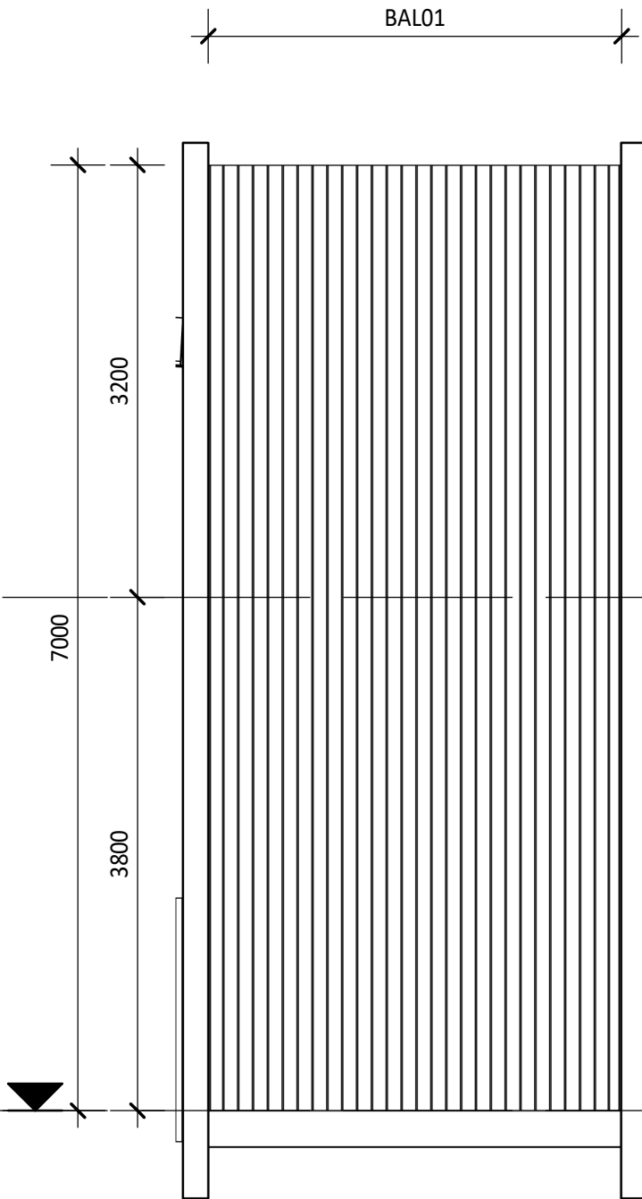
4 EXTERNAL STAIR SCREEN ELEVATION 44-03 1 : 50
